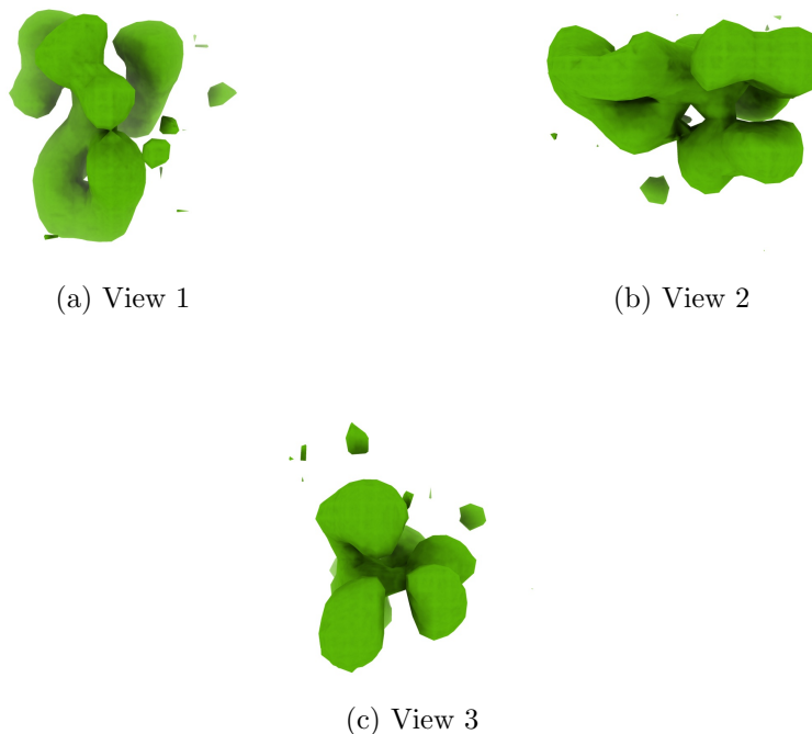
Figure 4: Isosurface at threshold=0.493000. Views generated by ChimeraX at a the following X, Y, Z angles: View 1 (0, -90, -90), View 2 (-90, 0, -90), View 3 (0, 0, 0).
