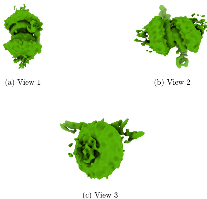
Figure 4: Isosurface at threshold=0.029000. Views generated by ChimeraX at a the following X, Y, Z angles: View 1 (0, -90, -90), View 2 (-90, 0, -90), View 3 (0, 0, 0).
