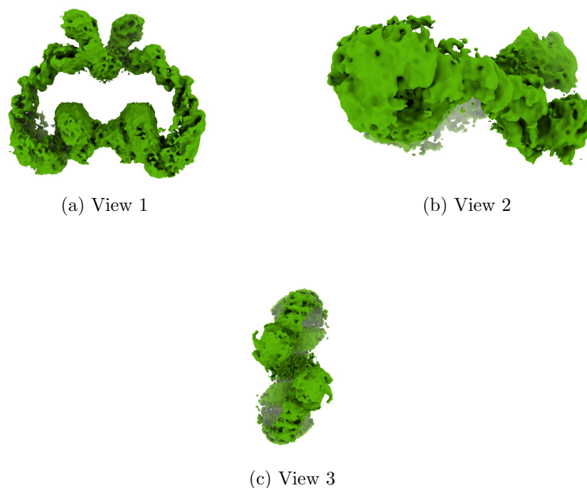
Figure 4: Isosurface at threshold=0.026100. Views generated by ChimeraX at a the following X, Y, Z angles: View 1 (0, -90, -90), View 2 (-90, 0, -90), View 3 (0, 0, 0).
