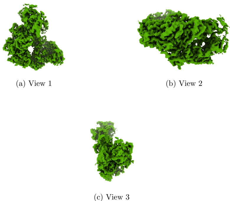
Figure 4: Isosurface at threshold=0.102000. Views generated by ChimeraX at a the following X, Y, Z angles: View 1 (0, -90, -90), View 2 (-90, 0, -90), View 3 (0, 0, 0).
