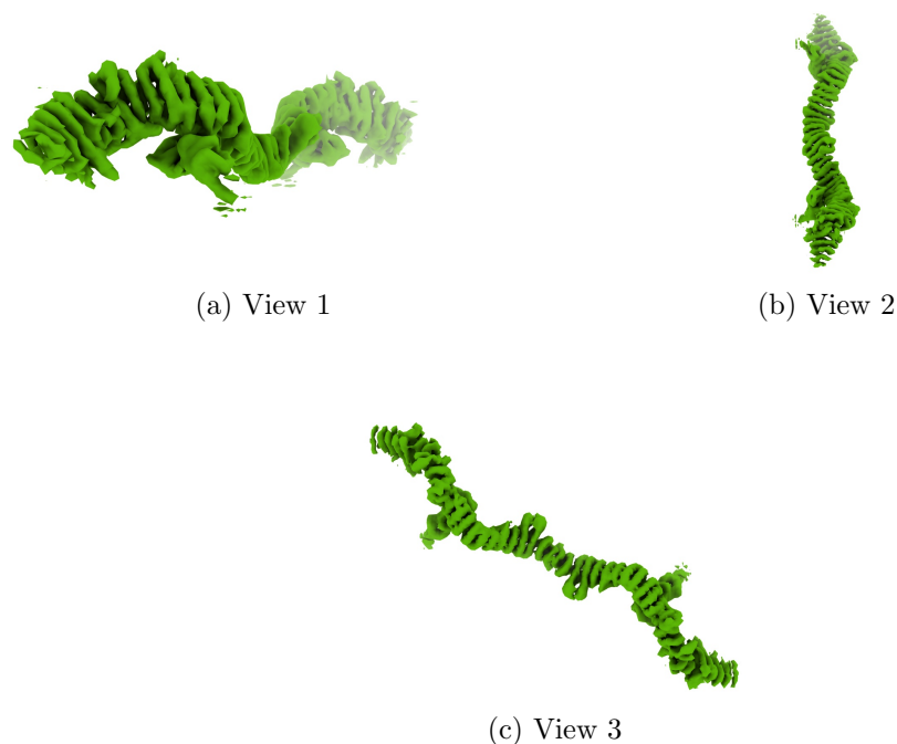
Figure 4: Isosurface at threshold=0.028000. Views generated by ChimeraX at a the following X, Y, Z angles: View 1 (0, -90, -90), View 2 (-90, 0, -90), View 3 (0, 0, 0).
