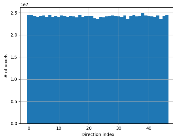
Figure 23: Histogram 1D of the best direction at each voxel.
