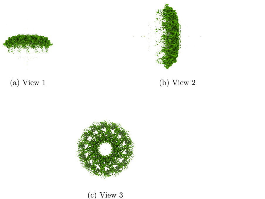
Figure 4: Isosurface at threshold=0.130000. Views generated by ChimeraX at a the following X, Y, Z angles: View 1 (0, -90, -90), View 2 (-90, 0, -90), View 3 (0, 0, 0).
