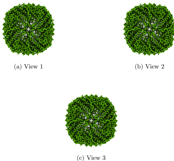
Figure 4: Isosurface at threshold=0.159000. Views generated by ChimeraX at a the following X, Y, Z angles: View 1 (0, -90, -90), View 2 (-90, 0, -90), View 3 (0, 0, 0).
