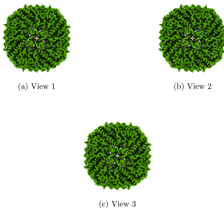
Figure 4: Isosurface at threshold=0.226000. Views generated by ChimeraX at a the following X, Y, Z angles: View 1 (0, -90, -90), View 2 (-90, 0, -90), View 3 (0, 0, 0).
