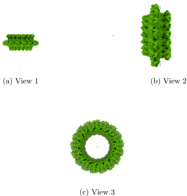
Figure 4: Isosurface at threshold=0.075000. Views generated by ChimeraX at a the following X, Y, Z angles: View 1 (0, -90, -90), View 2 (-90, 0, -90), View 3 (0, 0, 0).
