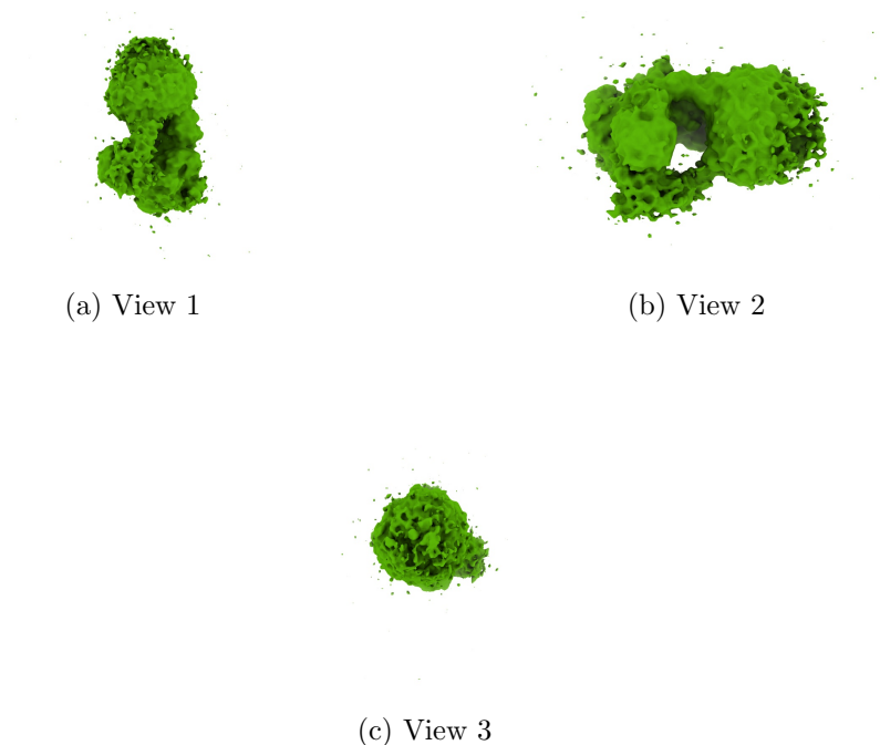
Figure 4: Isosurface at threshold=0.083900. Views generated by ChimeraX at a the following X, Y, Z angles: View 1 (0, -90, -90), View 2 (-90, 0, -90), View 3 (0, 0, 0).
