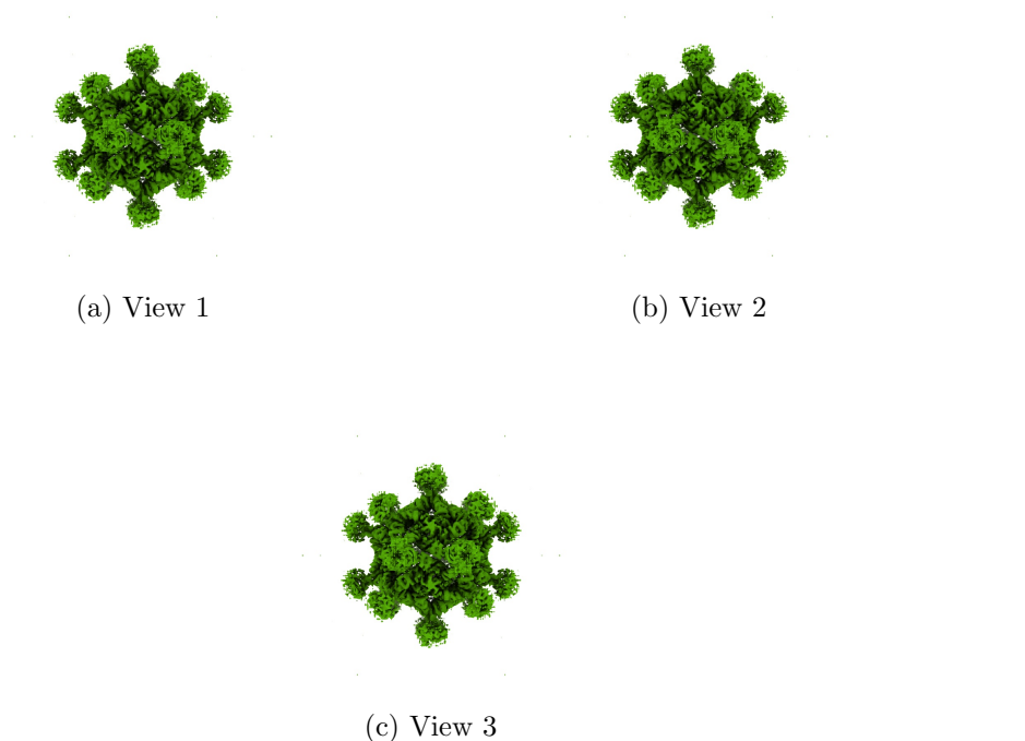
Figure 4: Isosurface at threshold=1.070000. Views generated by ChimeraX at a the following X, Y, Z angles: View 1 (0, -90, -90), View 2 (-90, 0, -90), View 3 (0, 0, 0).
