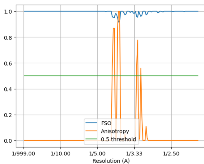
Figure 30: FSO and anisotropy.
