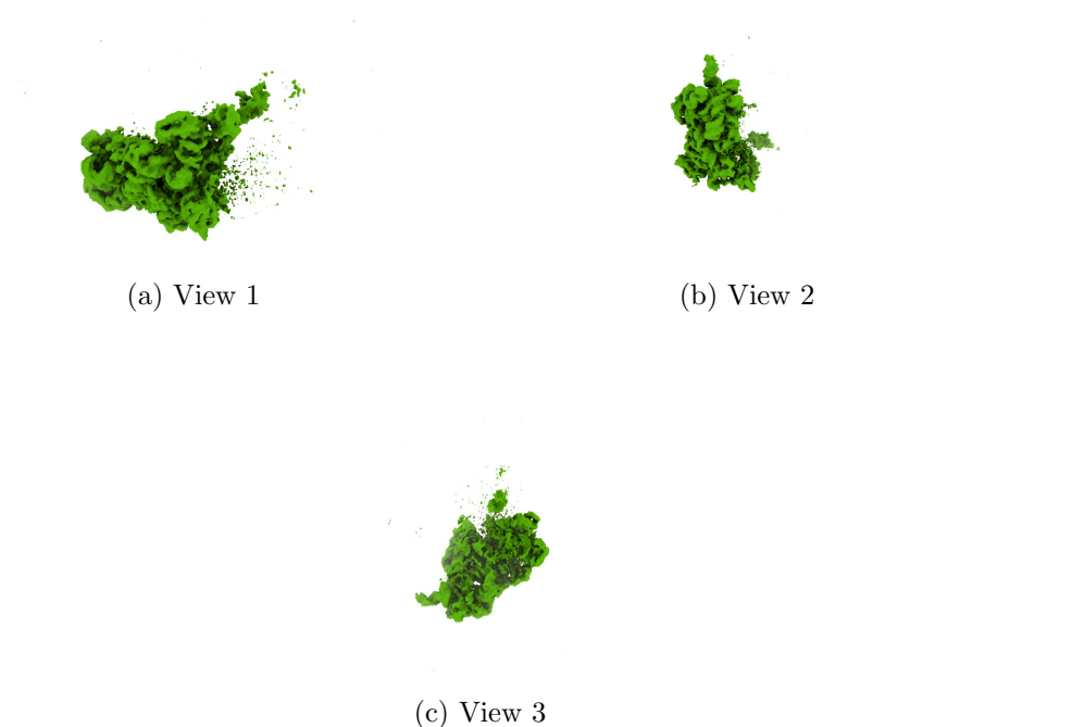
Figure 4: Isosurface at threshold=0.230000. Views generated by ChimeraX at a the following X, Y, Z angles: View 1 (0, -90, -90), View 2 (-90, 0, -90), View 3 (0, 0, 0).
