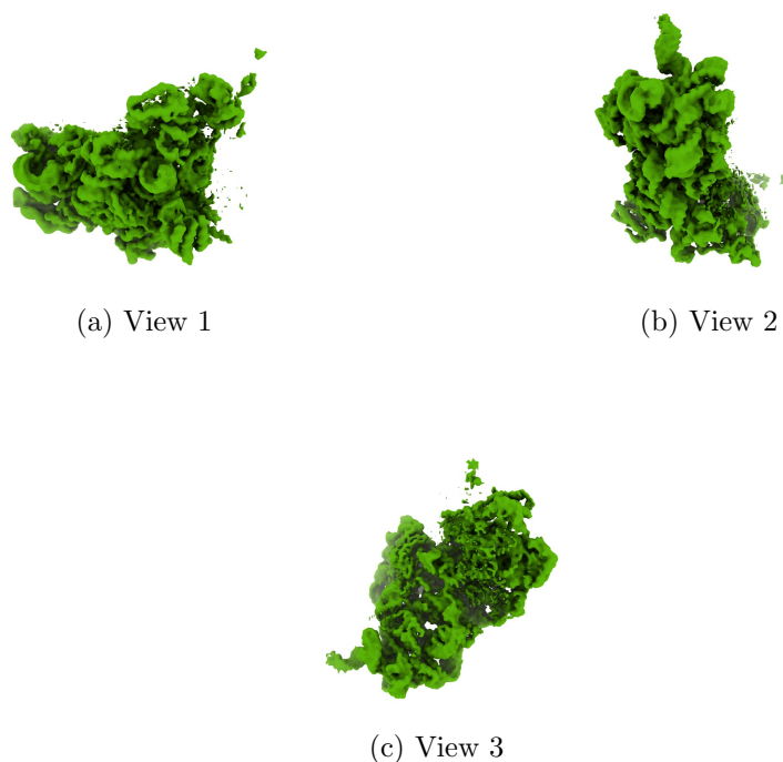
Figure 4: Isosurface at threshold=0.290000. Views generated by ChimeraX at a the following X, Y, Z angles: View 1 (0, -90, -90), View 2 (-90, 0, -90), View 3 (0, 0, 0).
