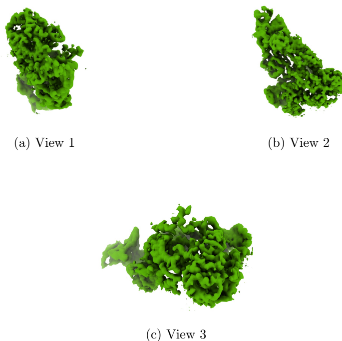
Figure 4: Isosurface at threshold=0.260000. Views generated by ChimeraX at a the following X, Y, Z angles: View 1 (0, -90, -90), View 2 (-90, 0, -90), View 3 (0, 0, 0).
