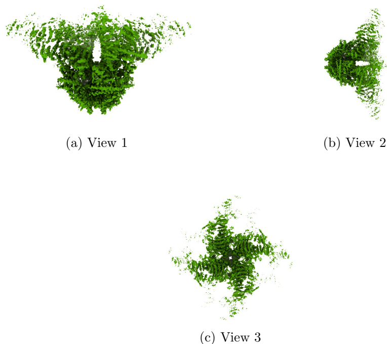
Figure 4: Isosurface at threshold=0.160000. Views generated by ChimeraX at a the following X, Y, Z angles: View 1 (0, -90, -90), View 2 (-90, 0, -90), View 3 (0, 0, 0).
