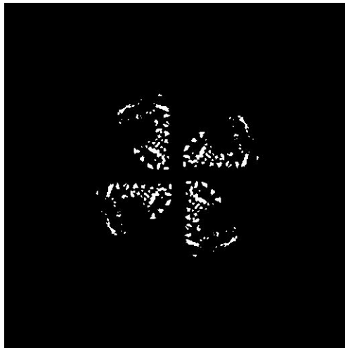
(c) Z Slice 233
