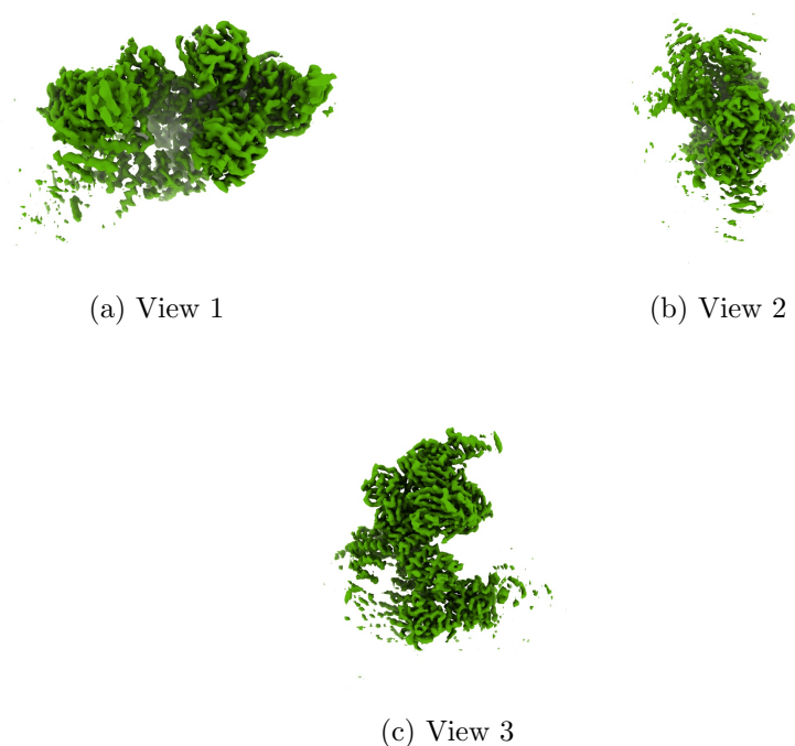
Figure 4: Isosurface at threshold=0.160000. Views generated by ChimeraX at a the following X, Y, Z angles: View 1 (0, -90, -90), View 2 (-90, 0, -90), View 3 (0, 0, 0).
