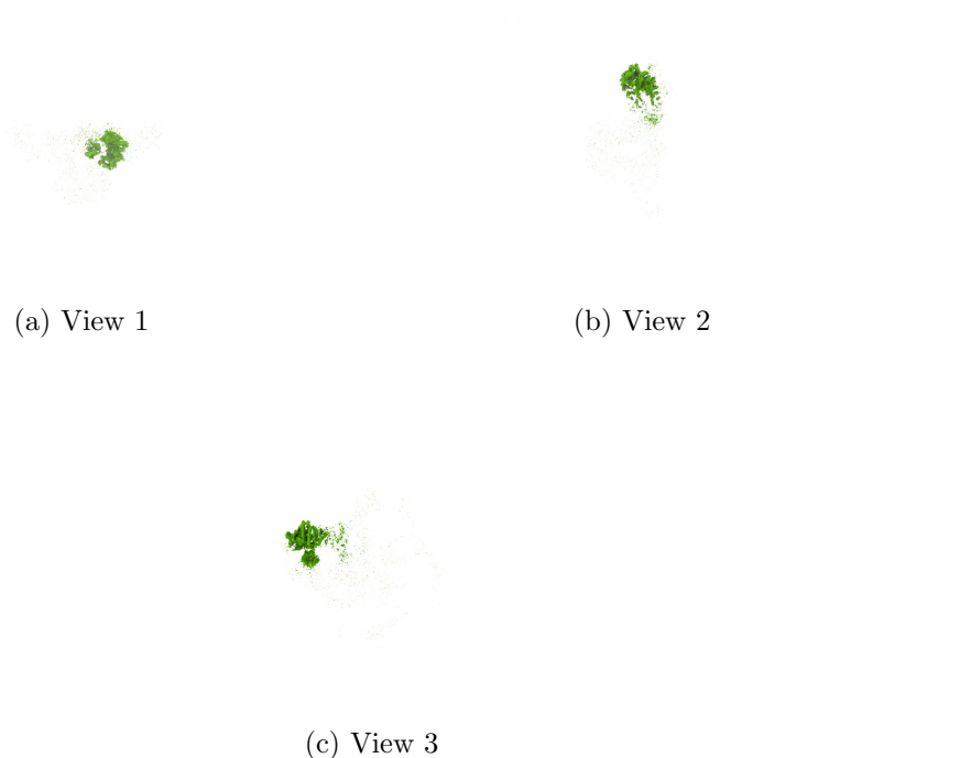
Figure 4: Isosurface at threshold=0.160000. Views generated by ChimeraX at a the following X, Y, Z angles: View 1 (0, -90, -90), View 2 (-90, 0, -90), View 3 (0, 0, 0).
