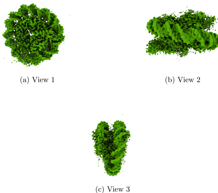
Figure 4: Isosurface at threshold=0.310000. Views generated by ChimeraX at a the following X, Y, Z angles: View 1 (0, -90, -90), View 2 (-90, 0, -90), View 3 (0, 0, 0).
