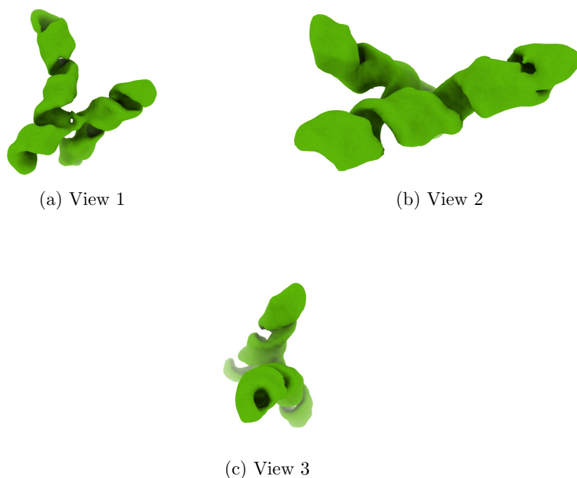
Figure 4: Isosurface at threshold=0.950000. Views generated by ChimeraX at a the following X, Y, Z angles: View 1 (0, -90, -90), View 2 (-90, 0, -90), View 3 (0, 0, 0).
