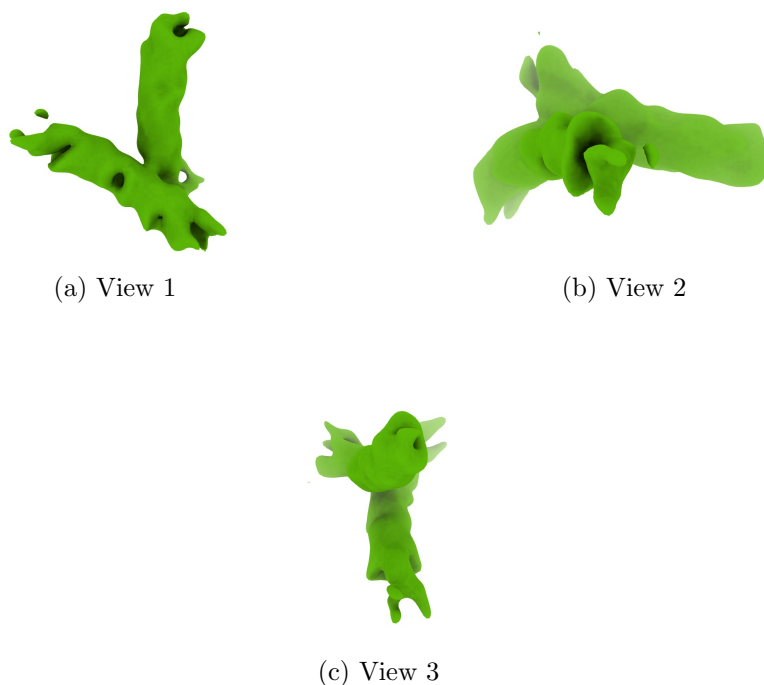
Figure 4: Isosurface at threshold=0.420000. Views generated by ChimeraX at a the following X, Y, Z angles: View 1 (0, -90, -90), View 2 (-90, 0, -90), View 3 (0, 0, 0).
