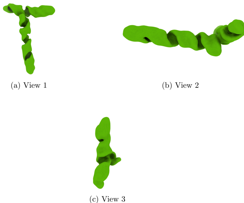
Figure 4: Isosurface at threshold=0.320000. Views generated by ChimeraX at a the following X, Y, Z angles: View 1 (0, -90, -90), View 2 (-90, 0, -90), View 3 (0, 0, 0).
