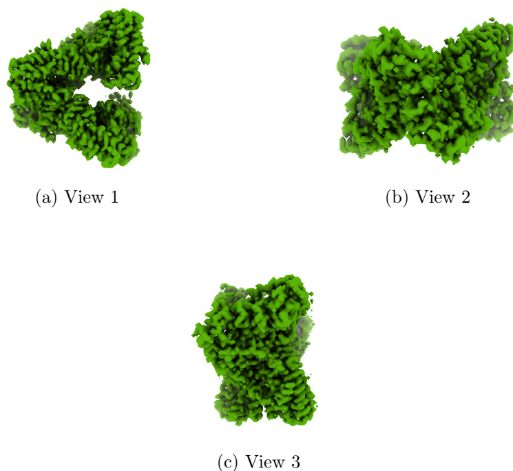
Figure 4: Isosurface at threshold=0.066000. Views generated by ChimeraX at a the following X, Y, Z angles: View 1 (0, -90, -90), View 2 (-90, 0, -90), View 3 (0, 0, 0).
