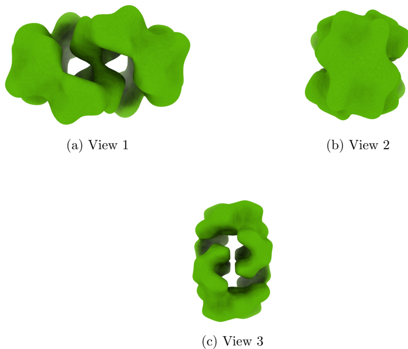
Figure 4: Isosurface at threshold=1.140000. Views generated by ChimeraX at a the following X, Y, Z angles: View 1 (0, -90, -90), View 2 (-90, 0, -90), View 3 (0, 0, 0).
