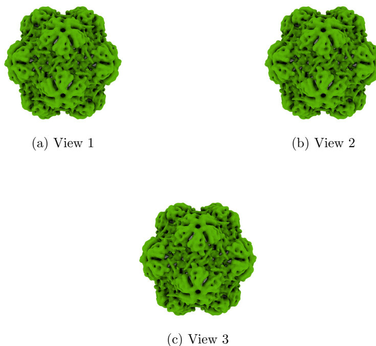
Figure 4: Isosurface at threshold=2.340000. Views generated by ChimeraX at a the following X, Y, Z angles: View 1 (0, -90, -90), View 2 (-90, 0, -90), View 3 (0, 0, 0).
