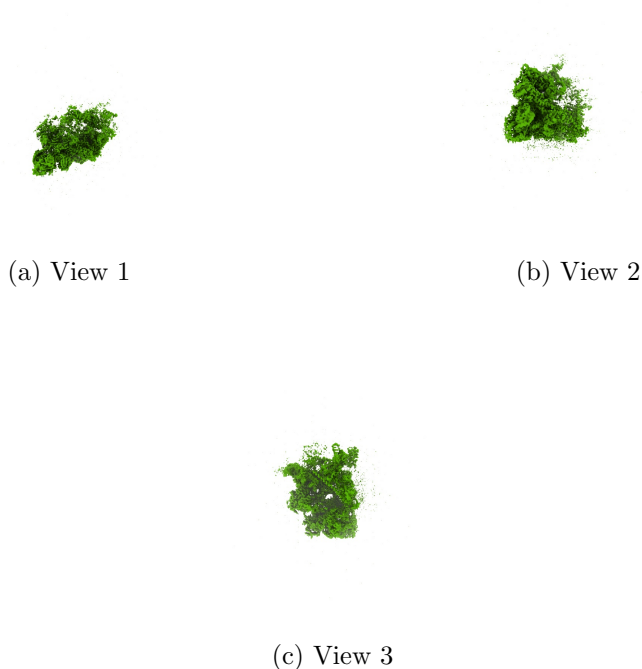
Figure 4: Isosurface at threshold=0.012000. Views generated by ChimeraX at a the following X, Y, Z angles: View 1 (0, -90, -90), View 2 (-90, 0, -90), View 3 (0, 0, 0).
