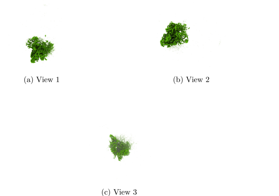
Figure 4: Isosurface at threshold=0.015000. Views generated by ChimeraX at a the following X, Y, Z angles: View 1 (0, -90, -90), View 2 (-90, 0, -90), View 3 (0, 0, 0).
