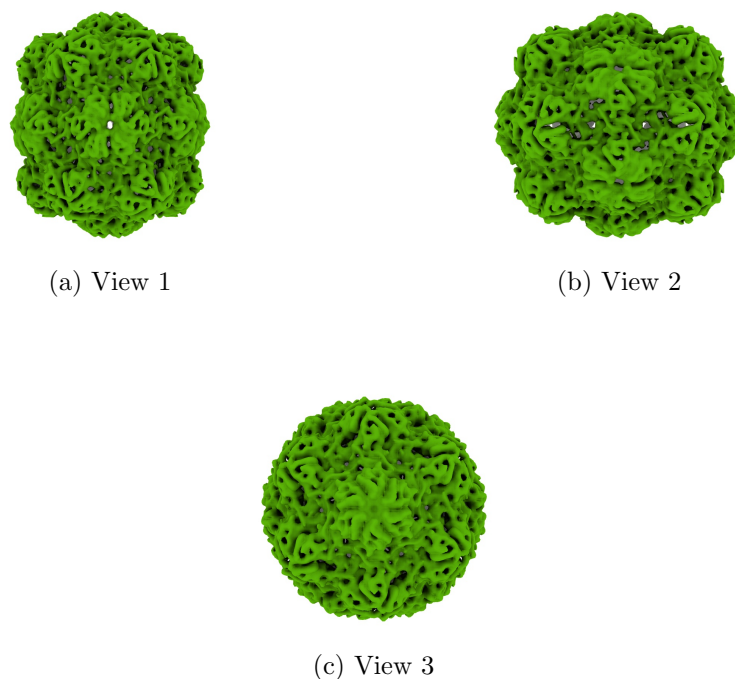
Figure 4: Isosurface at threshold=2.310000. Views generated by ChimeraX at the following X, Y, Z angles: View 1 (0, -90, -90), View 2 (-90, 0, -90), View 3 (0, 0, 0).
