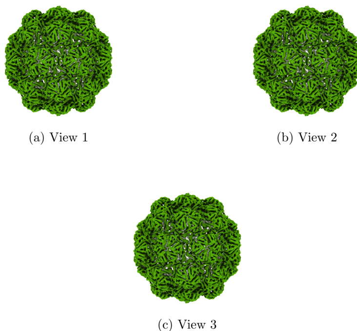
Figure 4: Isosurface at threshold=0.723000. Views generated by ChimeraX at a the following X, Y, Z angles: View 1 (0, -90, -90), View 2 (-90, 0, -90), View 3 (0, 0, 0).
