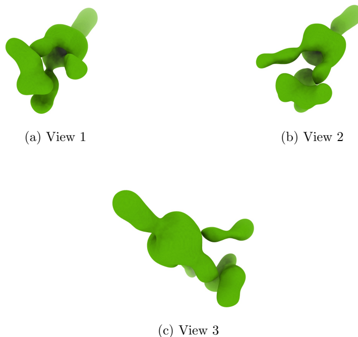
Figure 4: Isosurface at threshold=0.031100. Views generated by ChimeraX at a the following X, Y, Z angles: View 1 (0, -90, -90), View 2 (-90, 0, -90), View 3 (0, 0, 0).
