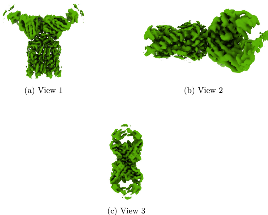
Figure 4: Isosurface at threshold=0.120000. Views generated by ChimeraX at a the following X, Y, Z angles: View 1 (0, -90, -90), View 2 (-90, 0, -90), View 3 (0, 0, 0).
