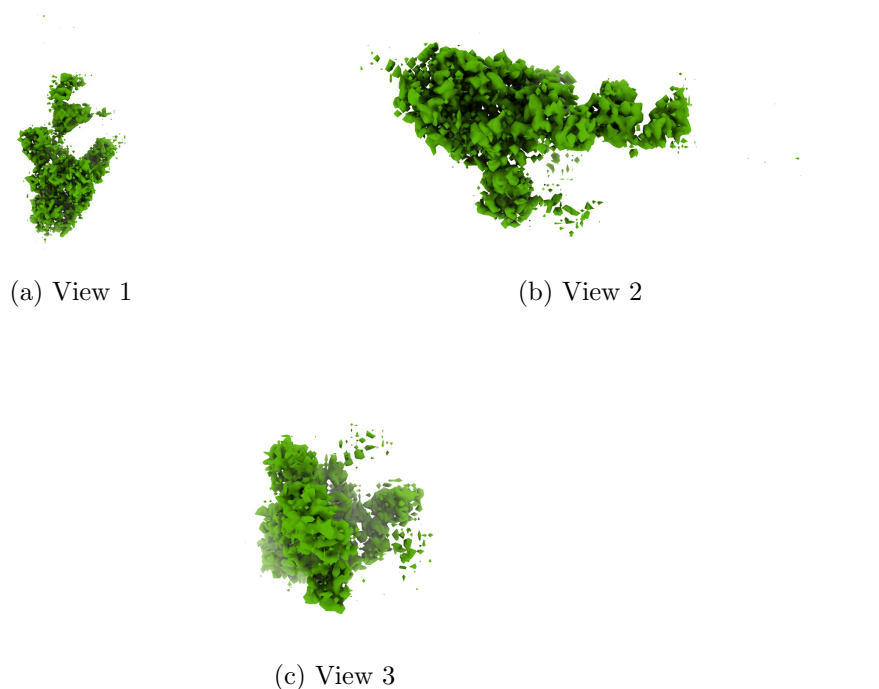
Figure 4: Isosurface at threshold=0.140000. Views generated by ChimeraX at a the following X, Y, Z angles: View 1 (0, -90, -90), View 2 (-90, 0, -90), View 3 (0, 0, 0).
