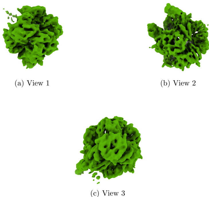
Figure 4: Isosurface at threshold=0.006840. Views generated by ChimeraX at a the following X, Y, Z angles: View 1 (0, -90, -90), View 2 (-90, 0, -90), View 3 (0, 0, 0).
