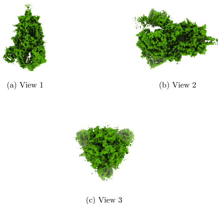
Figure 4: Isosurface at threshold=0.122000. Views generated by ChimeraX at a the following X, Y, Z angles: View 1 (0, -90, -90), View 2 (-90, 0, -90), View 3 (0, 0, 0).
