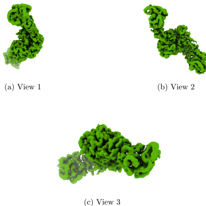
Figure 4: Isosurface at threshold=0.194000. Views generated by ChimeraX at a the following X, Y, Z angles: View 1 (0, -90, -90), View 2 (-90, 0, -90), View 3 (0, 0, 0).
