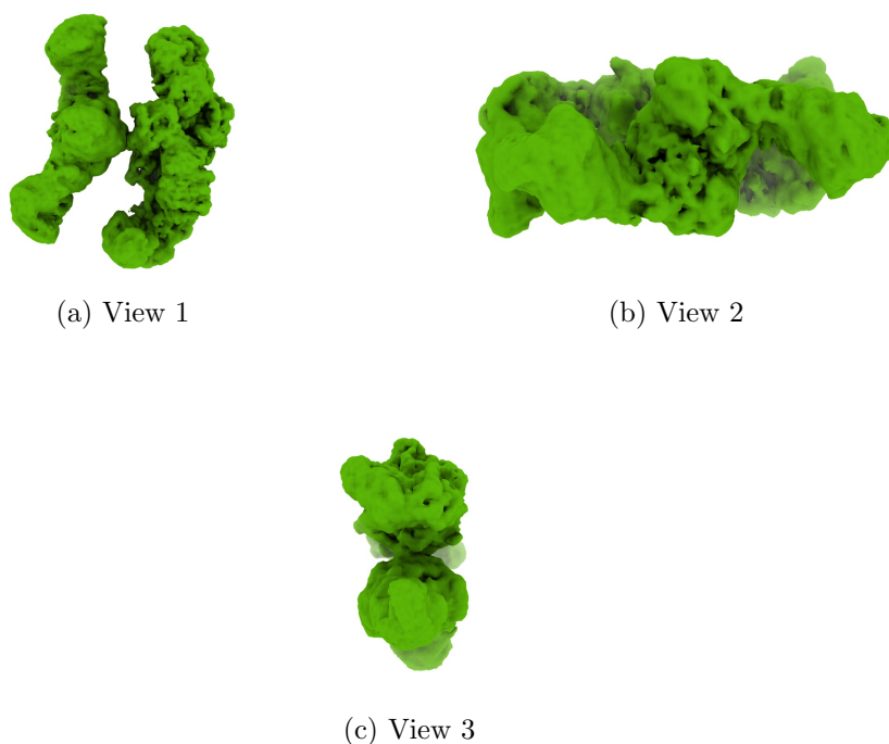
Figure 4: Isosurface at threshold=0.122000. Views generated by ChimeraX at a the following X, Y, Z angles: View 1 (0, -90, -90), View 2 (-90, 0, -90), View 3 (0, 0, 0).
