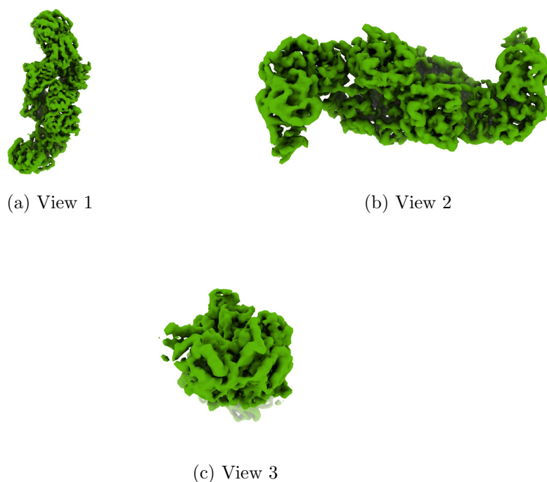
Figure 4: Isosurface at threshold=0.208000. Views generated by ChimeraX at a the following X, Y, Z angles: View 1 (0, -90, -90), View 2 (-90, 0, -90), View 3 (0, 0, 0).
