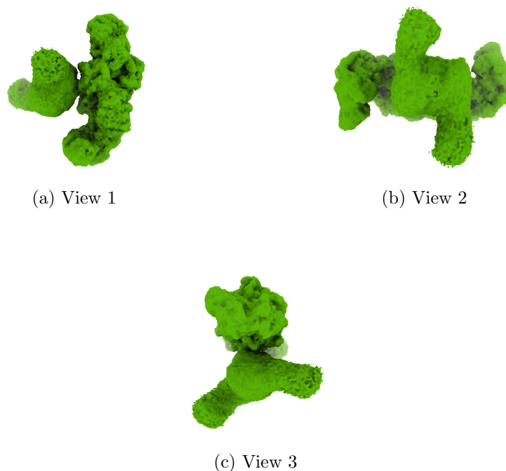
Figure 4: Isosurface at threshold=0.090100. Views generated by ChimeraX at a the following X, Y, Z angles: View 1 (0, -90, -90), View 2 (-90, 0, -90), View 3 (0, 0, 0).
