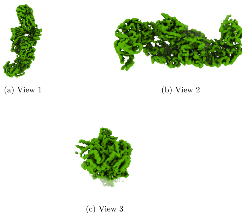
Figure 4: Isosurface at threshold=0.235000. Views generated by ChimeraX at a the following X, Y, Z angles: View 1 (0, -90, -90), View 2 (-90, 0, -90), View 3 (0, 0, 0).
