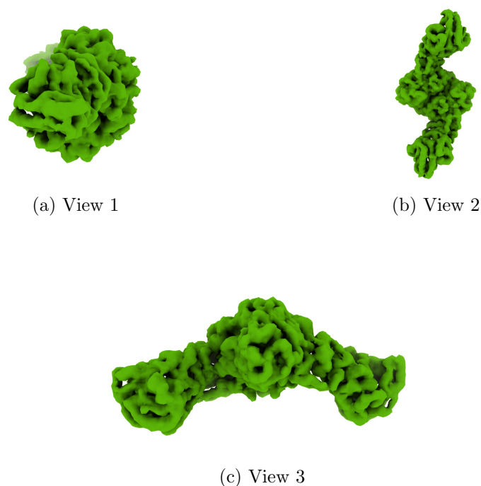
Figure 4: Isosurface at threshold=0.149000. Views generated by ChimeraX at a the following X, Y, Z angles: View 1 (0, -90, -90), View 2 (-90, 0, -90), View 3 (0, 0, 0).
