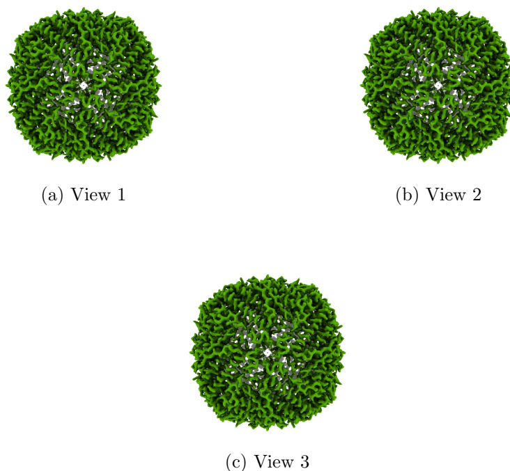
Figure 4: Isosurface at threshold=0.146000. Views generated by ChimeraX at a the following X, Y, Z angles: View 1 (0, -90, -90), View 2 (-90, 0, -90), View 3 (0, 0, 0).
