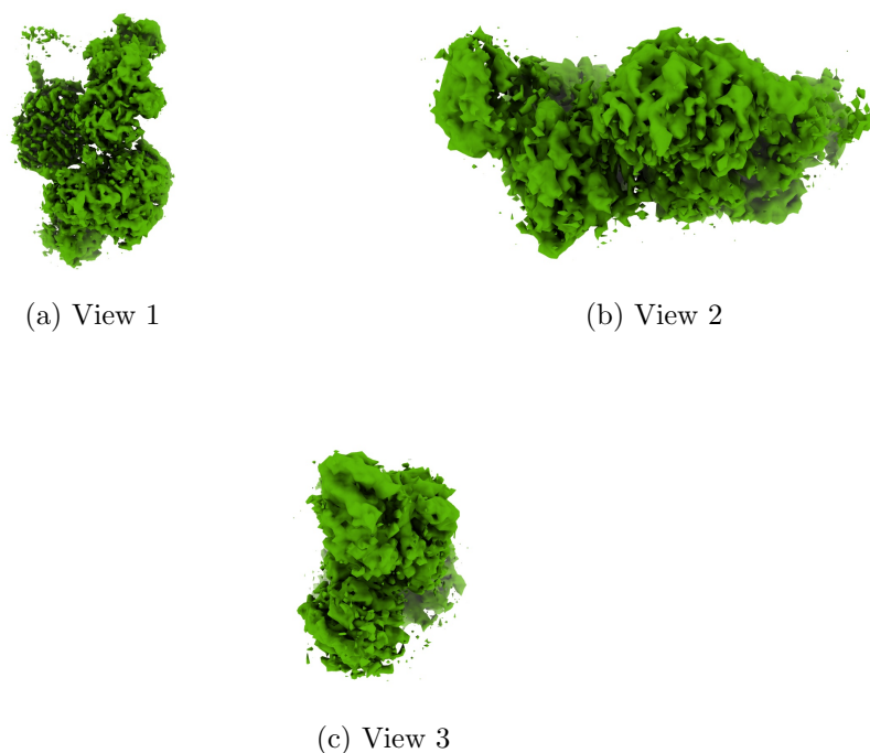
Figure 4: Isosurface at threshold=0.122000. Views generated by ChimeraX at a the following X, Y, Z angles: View 1 (0, -90, -90), View 2 (-90, 0, -90), View 3 (0, 0, 0).
