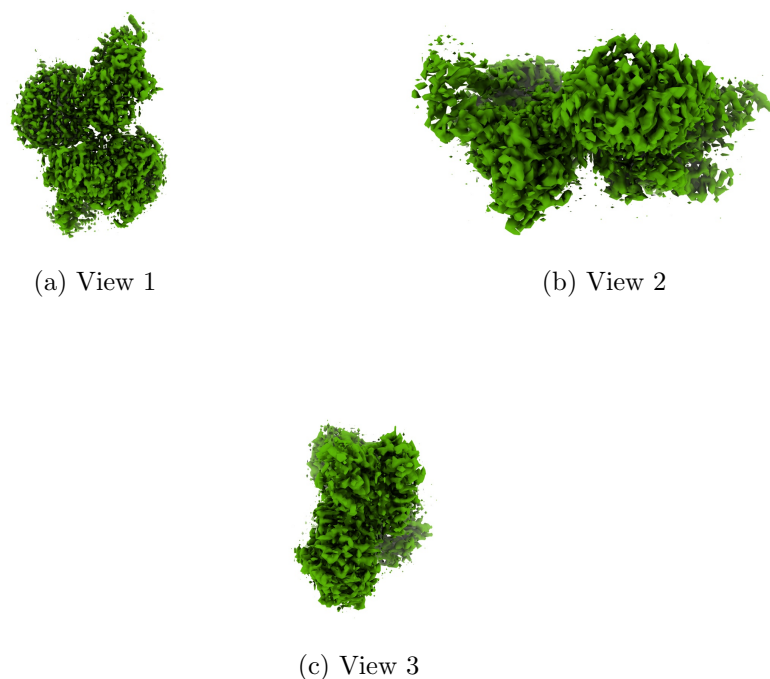
Figure 4: Isosurface at threshold=0.096700. Views generated by ChimeraX at a the following X, Y, Z angles: View 1 (0, -90, -90), View 2 (-90, 0, -90), View 3 (0, 0, 0).
