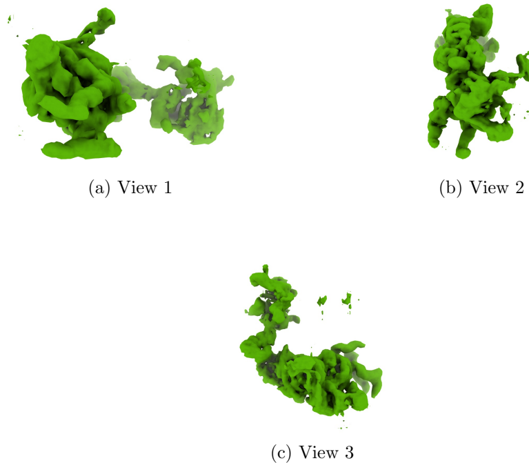
Figure 4: Isosurface at threshold=0.020800. Views generated by ChimeraX at a the following X, Y, Z angles: View 1 (0, -90, -90), View 2 (-90, 0, -90), View 3 (0, 0, 0).
