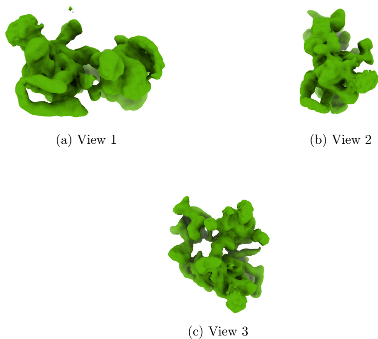
Figure 4: Isosurface at threshold=0.014900. Views generated by ChimeraX at a the following X, Y, Z angles: View 1 (0, -90, -90), View 2 (-90, 0, -90), View 3 (0, 0, 0).
