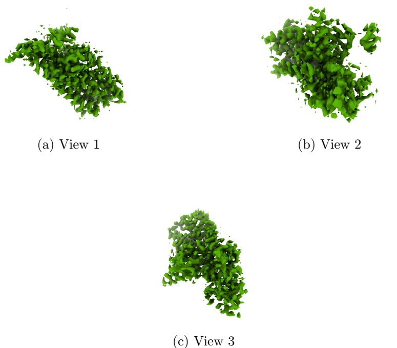
Figure 4: Isosurface at threshold=0.720000. Views generated by ChimeraX at a the following X, Y, Z angles: View 1 (0, -90, -90), View 2 (-90, 0, -90), View 3 (0, 0, 0).
