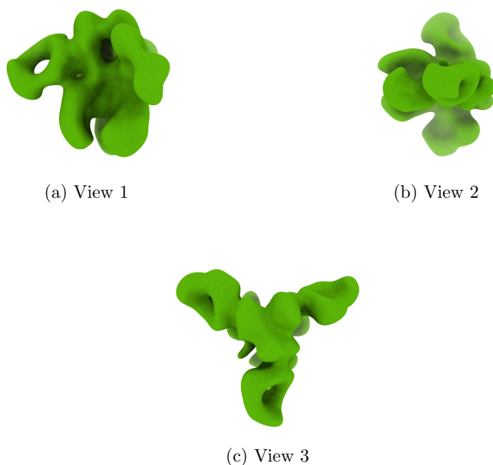
Figure 4: Isosurface at threshold=0.021400. Views generated by ChimeraX at a the following X, Y, Z angles: View 1 (0, -90, -90), View 2 (-90, 0, -90), View 3 (0, 0, 0).
