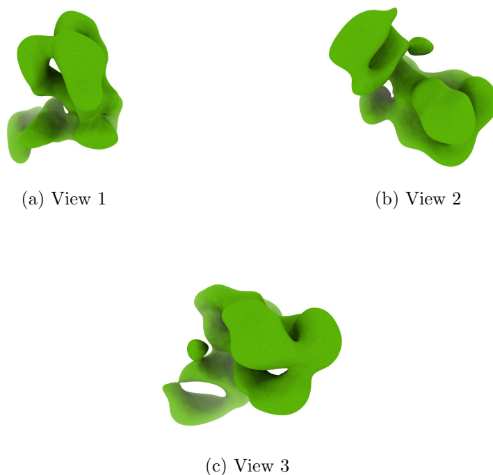
Figure 4: Isosurface at threshold=0.011800. Views generated by ChimeraX at a the following X, Y, Z angles: View 1 (0, -90, -90), View 2 (-90, 0, -90), View 3 (0, 0, 0).
