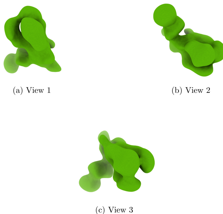
Figure 4: Isosurface at threshold=0.012100. Views generated by ChimeraX at a the following X, Y, Z angles: View 1 (0, -90, -90), View 2 (-90, 0, -90), View 3 (0, 0, 0).
